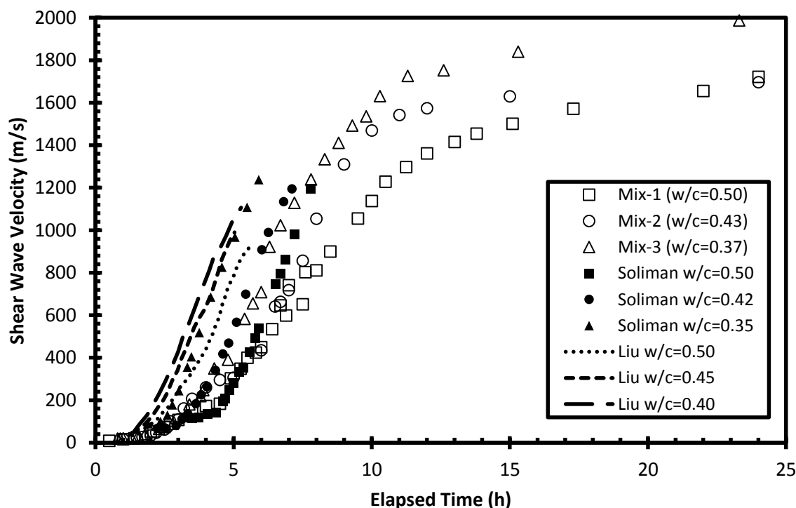
Figure 5.8. Comparison of Shear Wave Velocity Results
