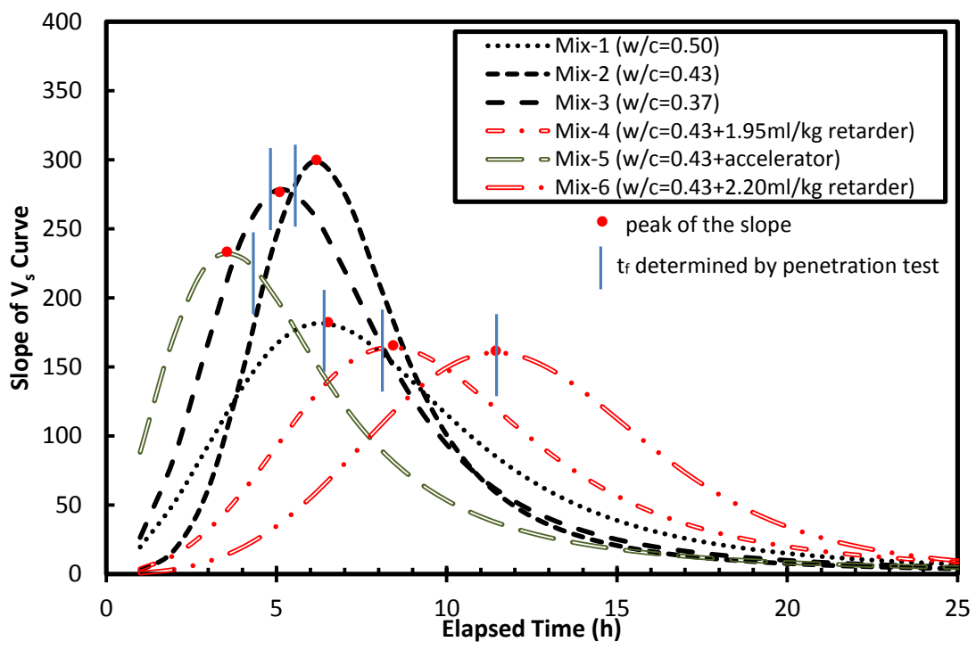
Figure 5.12. Slope of V_s versus Time
