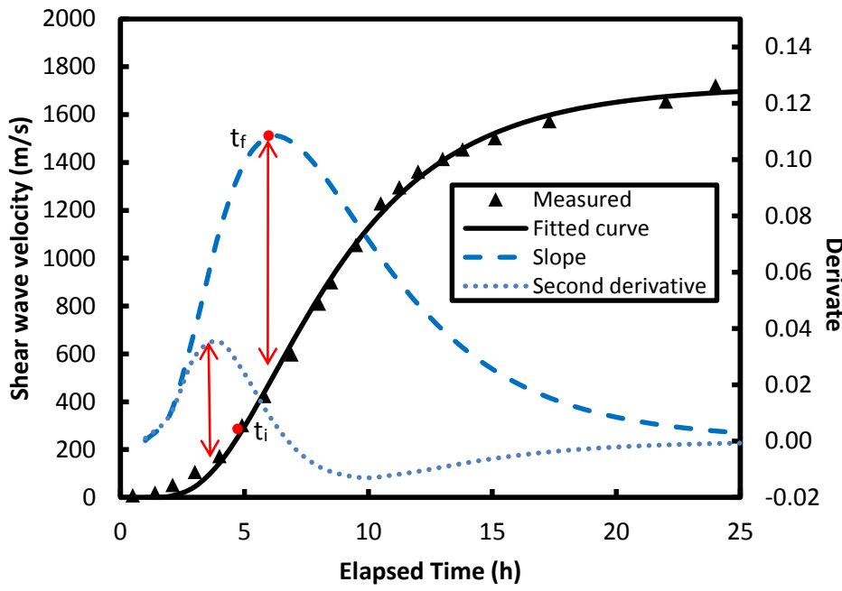
Figure 5.11. Slope and Second Derivative of V_s Curves
