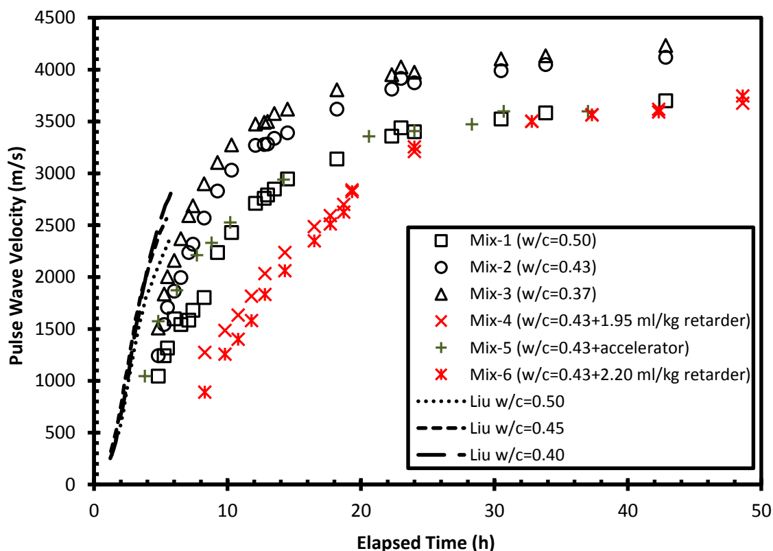
Figure 5.16. Pulse Wave Velocity versus Elapsed Time
